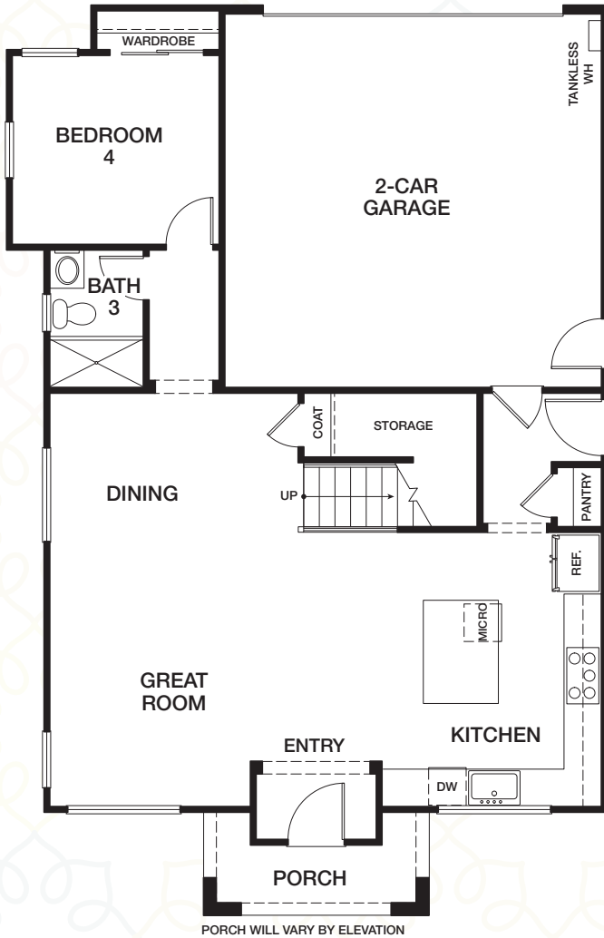
FIRST FLOOR
