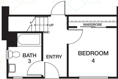
FIRST FLOOR ACCESSIBLE
