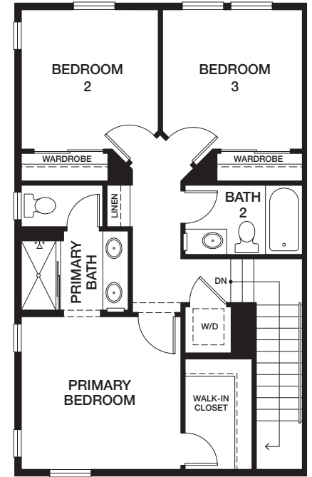
THIRD FLOOR
